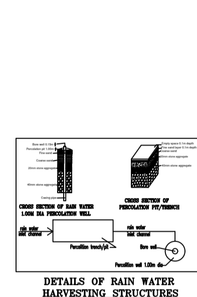
DETAILS OF RAIN WATER HARVESTING STRUCTURES
